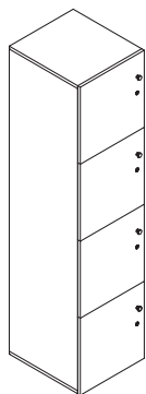
Locker LK45C 1x4 L: 45, W: 50, H: 190 cm
