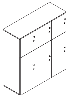
Locker LK45/90C 3x2 L: 135, W: 50, H: 145 cm
