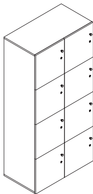
Locker LK45C 2x4 L: 90, W: 50, H: 190 cm
